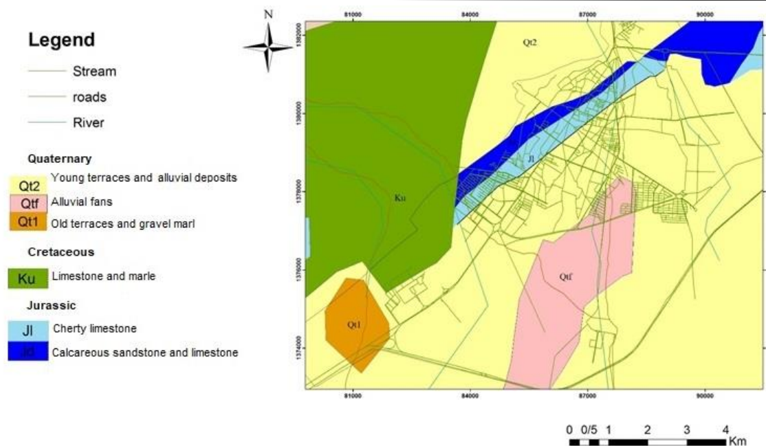
Fig. 2. The geological map of the study area
