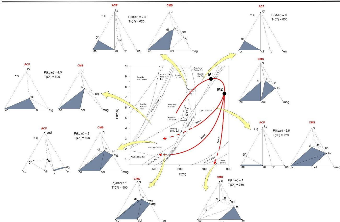
Fig. 7. The SCM and ACF diagrams calculated for the various P and T during metamorphism of the Qori complex dolomitic marbles.
