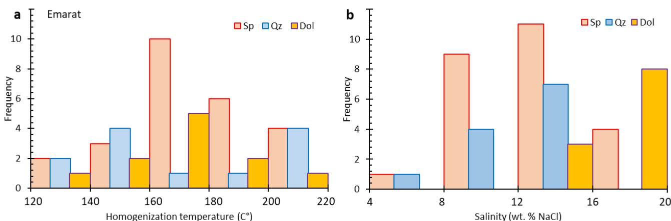
Fig. 10. Histograms of a) homogenization temperatures and b) salinities of fluid inclusions in sphalerite (Sp), quartz (Qz), and dolomite (Dol) from Emarat.
