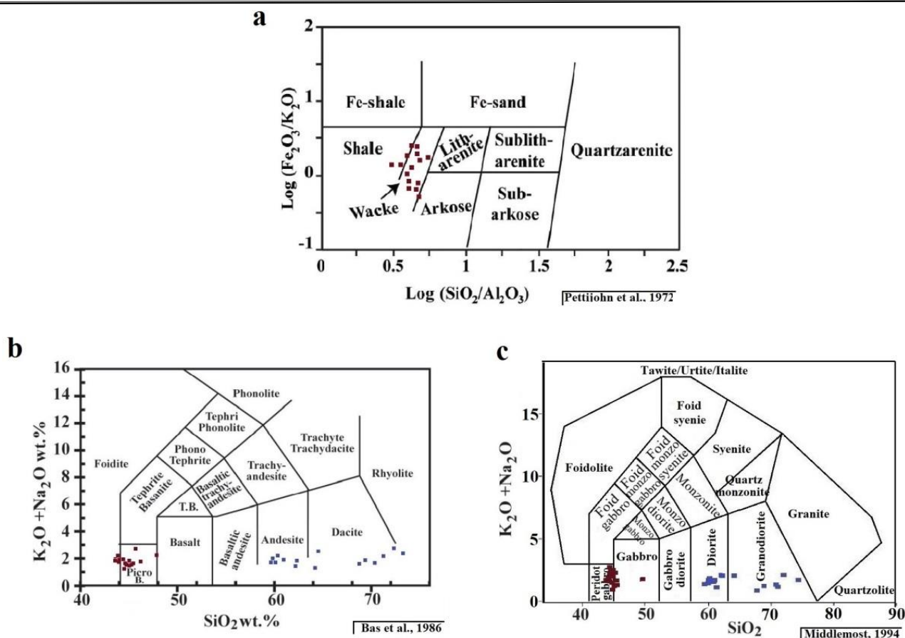
Fig. 8. a) Identifying the location of deposits in sedimentary rocks, b, c) The location of igneous rocks equivalent to the samples based on the main oxides
