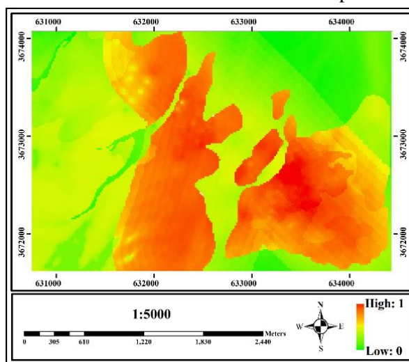
Fig. 3. Output of Fuzzy gamma operator (WGS 84 / UTM zone 39N).
