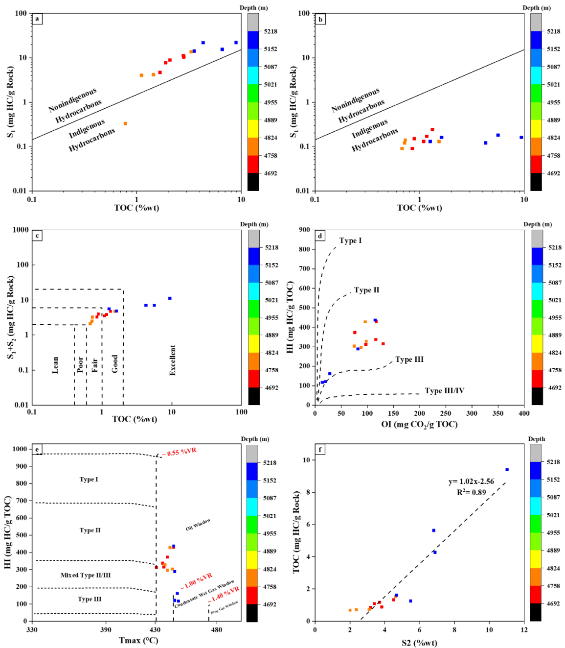
Fig. 2. a) Migration index plot used to assess sample contamination before washing with an organic solvent; b) after washing with an organic solvent (adopted from Hunt,1996); c) S_1+S_2 vs. TOC diagram for evaluating the hydrocarbon potential (adopted from Dembicki, 2009); d) HI vs. OI plot for determining type of kerogen (adopted from Hunt,1996); e) HI vs. Tmax plot (adopted from Abeed et al., 2011); f) TOC vs. S_2 diagram determining the inert and adsorbed carbon content of the Garau Formation samples
